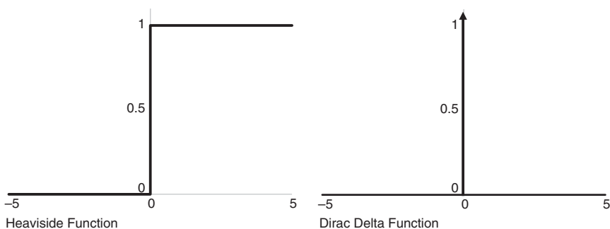
FIGURE 11.6 Heaviside and Dirac Delta Functions
